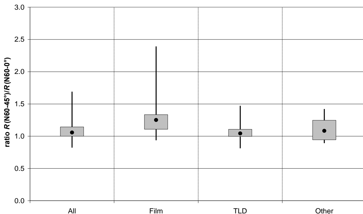
Figure 12. Ratios of H_p(10) responses for N60-45° and N60-0° (relative angular response). Dots: median ratios; bars: 25th to 75th percentiles; lines: 2.5th to 97.5th percentiles.
